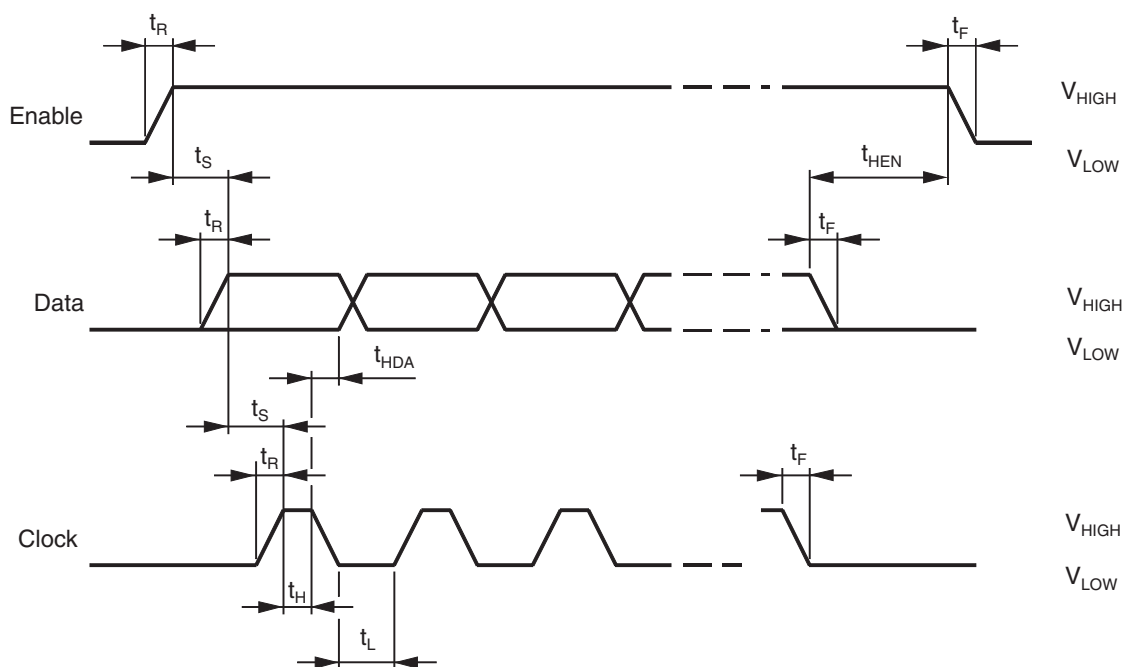
Figure 6-2. 3-wire Pulse Diagram
