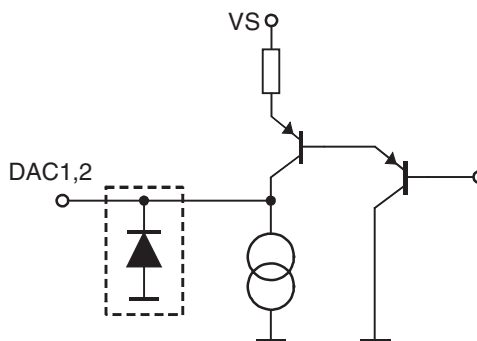
Figure 4-5. Internal Components at DAC1 and DAC2 Output
