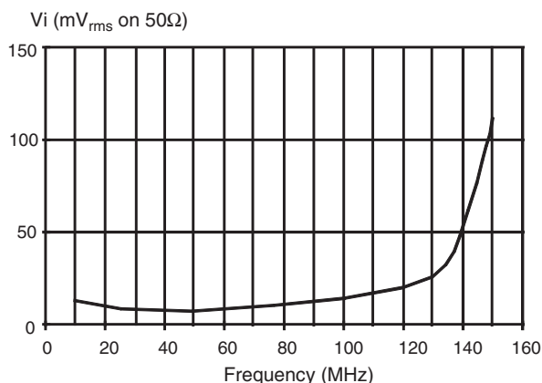
Figure 5-1. FMOSCIN Sensitivity
