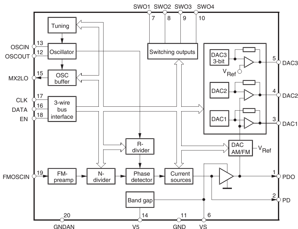
Figure 1-1. Block Diagram
